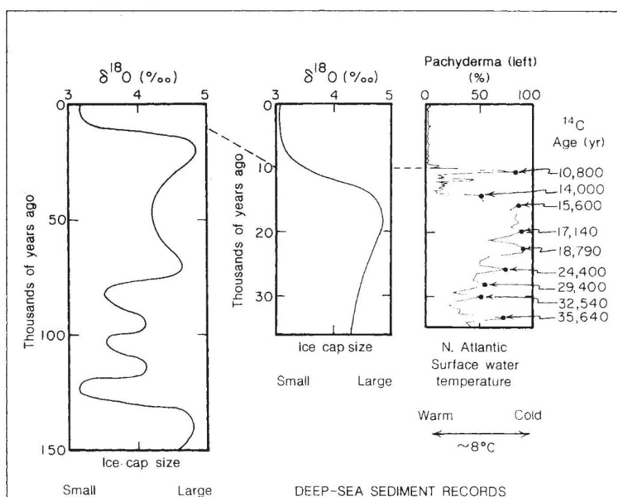
Fig. 1 The ratio of heavy oxygen ( ^{18}\text{O} ) to light oxygen ( ^{16}\text{O} ) in foraminifera shells preserved in deep-sea sediments provides our best record as to how the great continental ice sheets of the Northern Hemisphere waxed and waned. The reason is that the snow that builds ice caps is depleted in the heavy oxygen isotope. Therefore as ice caps grow, the ocean is correspondingly enriched in heavy oxygen. So also is the oxygen in the calcium carbonate of shells living in these waters.
