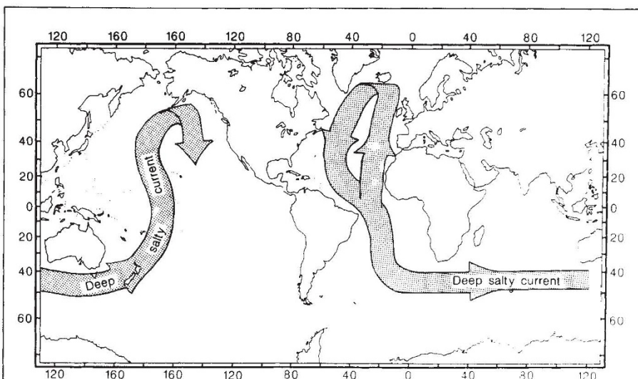
Fig. 2 A large-scale salt transport system operates in today's ocean to compensate for the transport of water (as vapour) through the atmosphere from the Atlantic to the Pacific Ocean. Salty, deep water formed in the North Atlantic flows down the length of the Atlantic, around Africa, through the southern Indian Ocean and finally northward in the deep Pacific Ocean. Some of this water upwells in the North Pacific, bringing with it the salt left behind in the Atlantic due to vapour transport. This atmospheric water vapour and ocean salt transport system is self-stabilizing. Records from ice and sediment tell us that this great conveyor system was somehow disrupted during glacial time and replaced by an alternative mode of operation.
